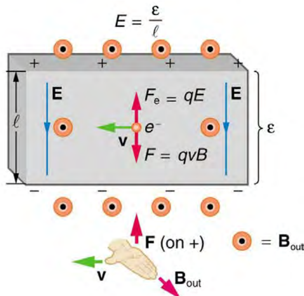
Figure 22.28 The Hall emf \epsilon produces an electric force that balances the magnetic force on the moving charges. The magnetic force produces charge separation, which builds up until it is balanced by the electric force, an equilibrium that is quickly reached.
