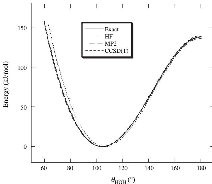
Figure 11.13 Angle bending curves for H 2 O
