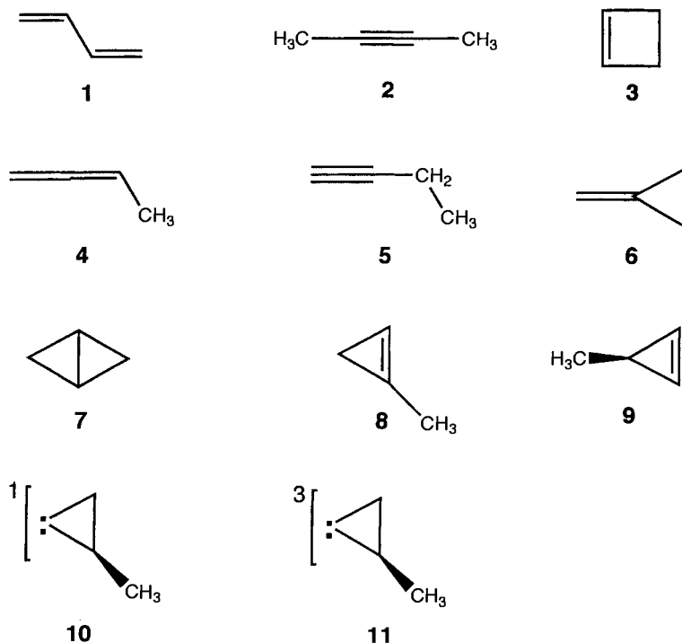
Figure 11.14 \text{C}_4\text{H}_6 isomers
