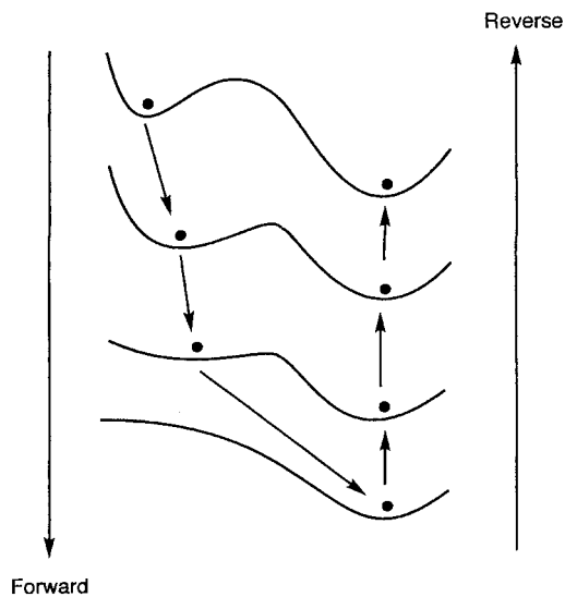
Figure 12.13 Illustration of the diffusion method
