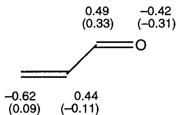
Figure 15.2 AM1 LUMO coefficients for acrolein with net charges in parenthesis
