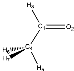
Figure D.1 Atom numbering for acetaldehyde
