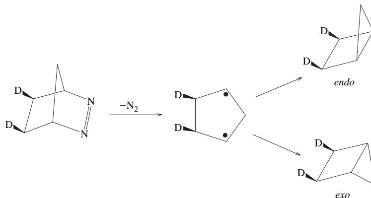
Figure 13.2 Thermal decomposition leads to a 4 : 1 preference for the exo isomer
