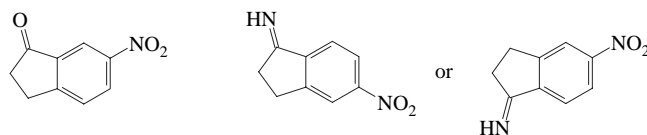
Figure 17.4 Illustrating the alignment problem in COMFA methods
