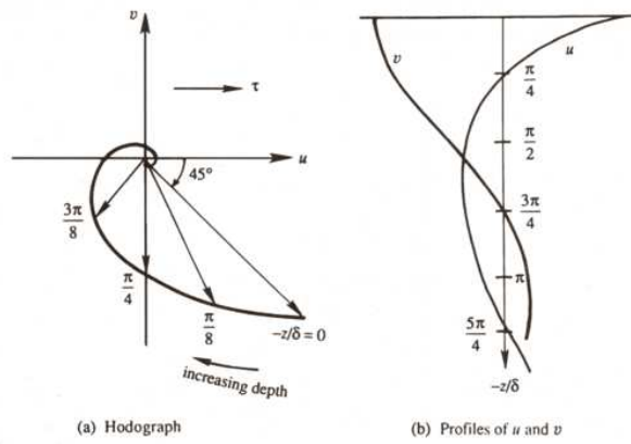
Figure 8.2: Ekman spiral for the ocean surface layer. This figure has been taken from Kundu and Cohen [2002].
