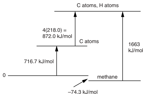
Figure 3-3 Enthalpy Diagram for the Atomization of Methane.
