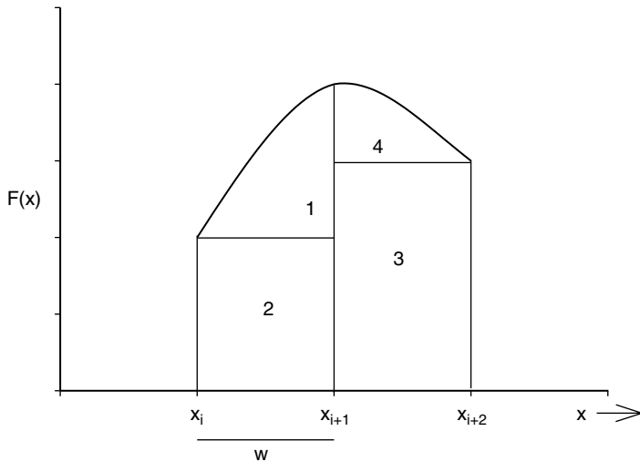
Figure 1-3 Areas Under a Parabolic Arc Covering Two Subintervals of a Simpson's Rule Integration.
