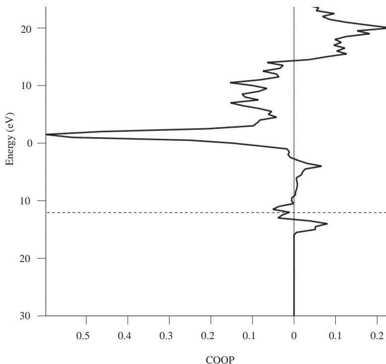
FIGURE 34.3 Crystal orbital overlap plot for CoNb 4 Si.
