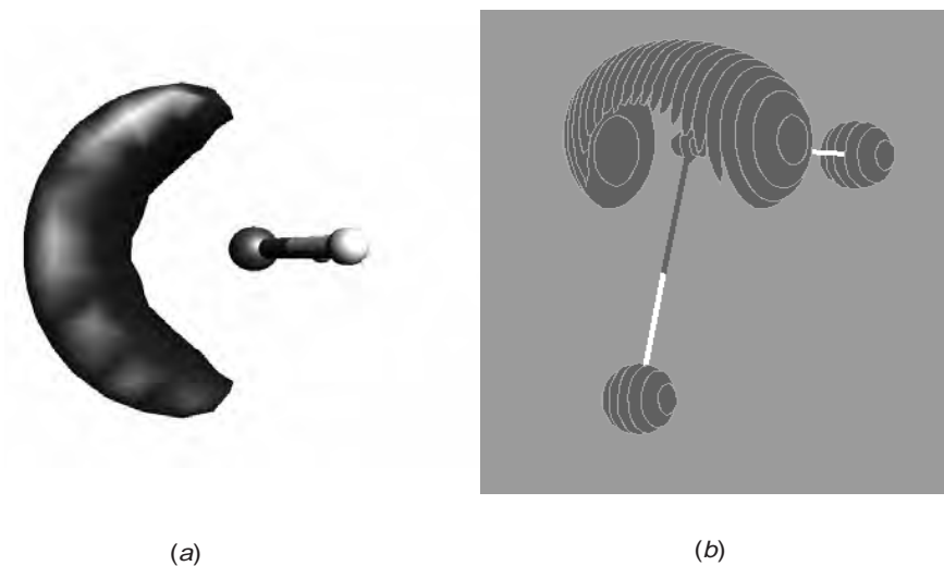
FIGURE 13.5 Isosurface plots. (a) Region of negative electrostatic potential around the water molecule. (b) Region where the Laplacian of the electron density is negative. Both of these plots have been proposed as descriptors of the lone-pair electrons. This example is typical in that the shapes of these regions are similar, but the Laplacian region tends to be closer to the nucleus.
