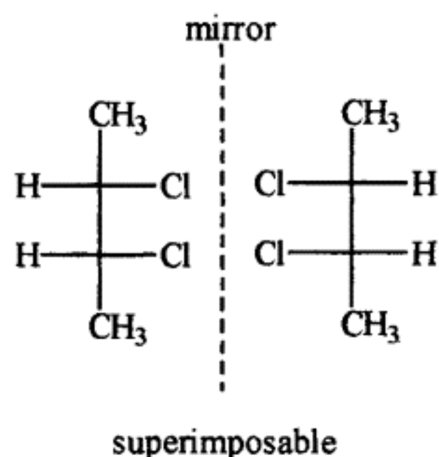
Figure 3.5. Meso Compound
