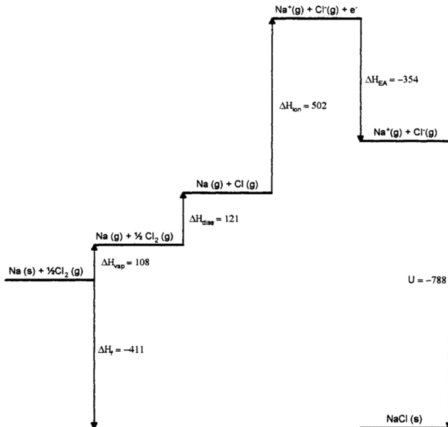
Figure 2.4. Born-Haber Cycle
