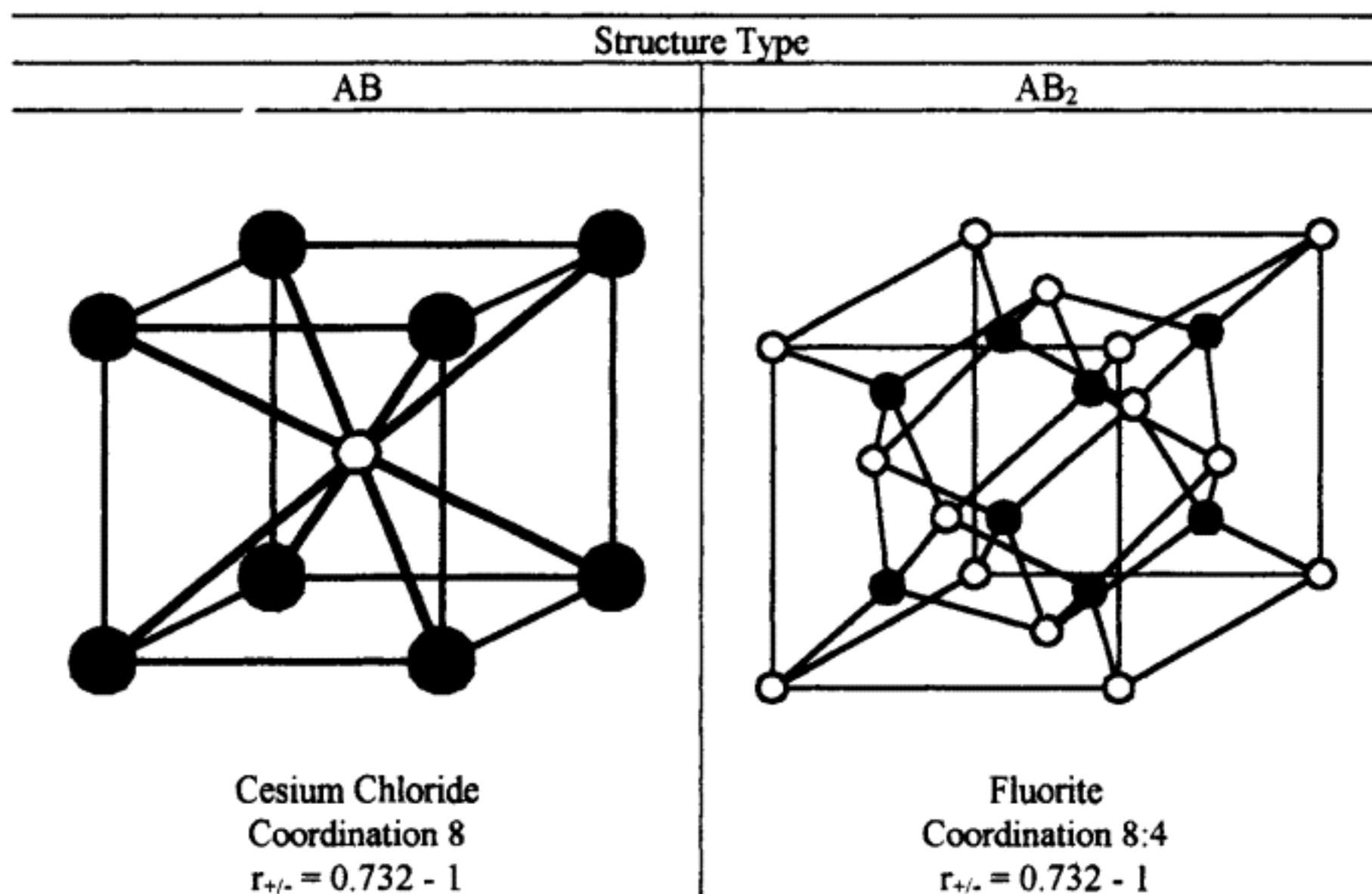
Figure 2.3. Common Lattice Types
