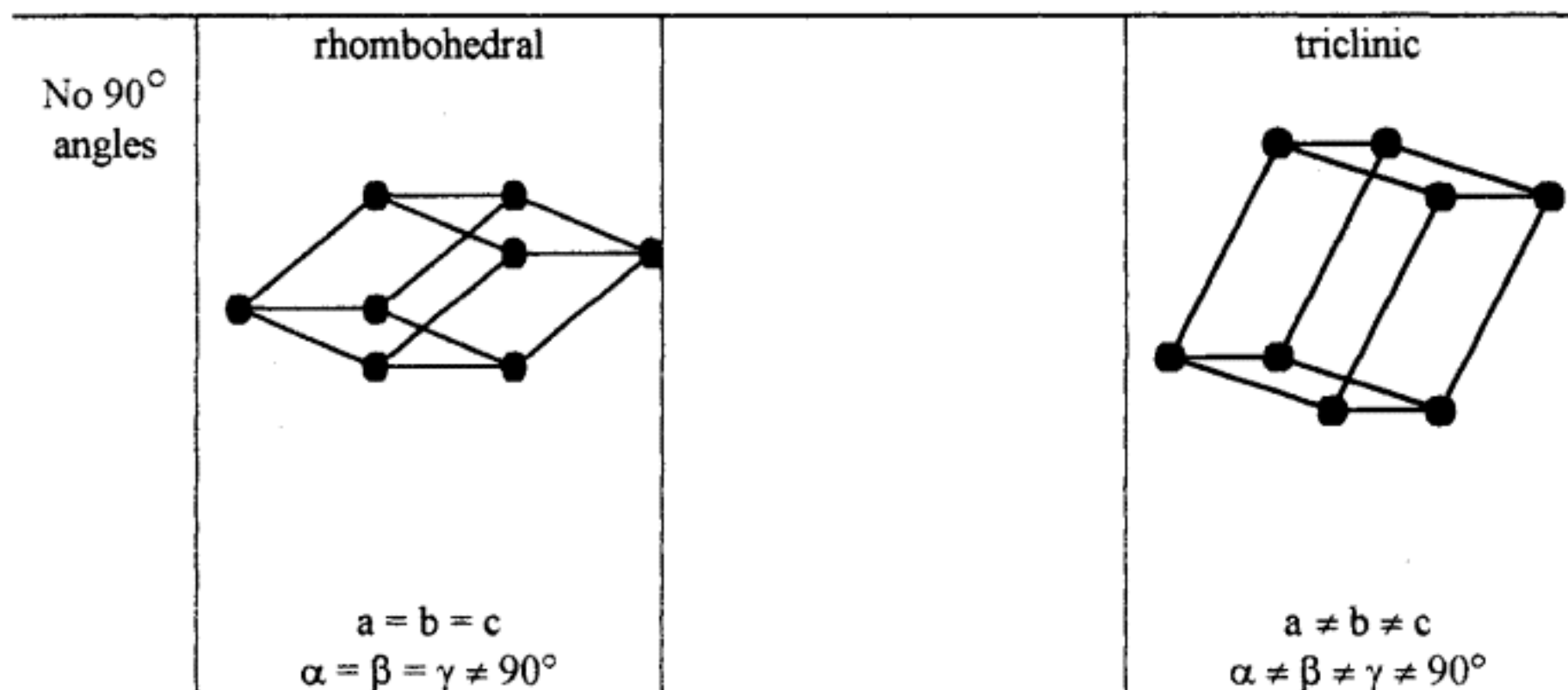
Figure 2.1. Unit Cells
