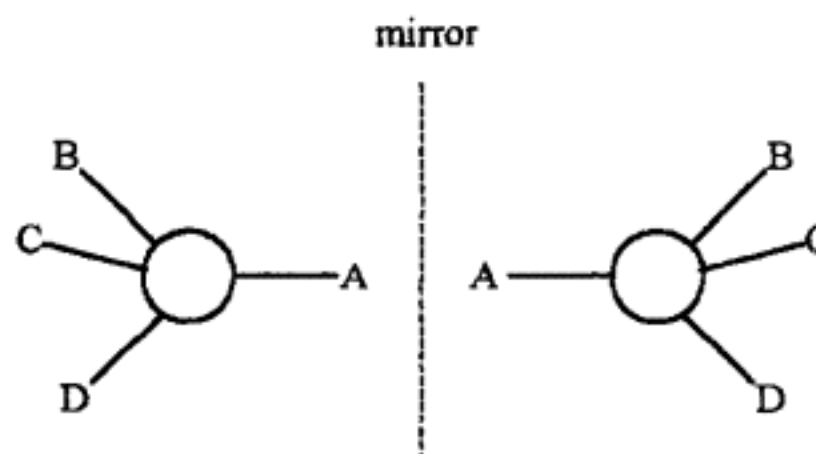
Figure 3.3. Enantiomers
