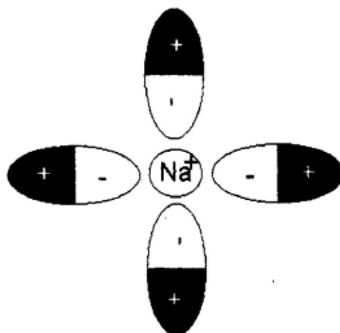
Figure 1.7. Ion-dipole attraction
