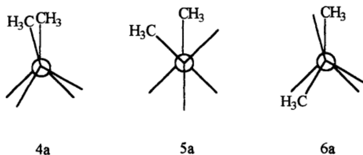
Figure 3.12. Newman projections
