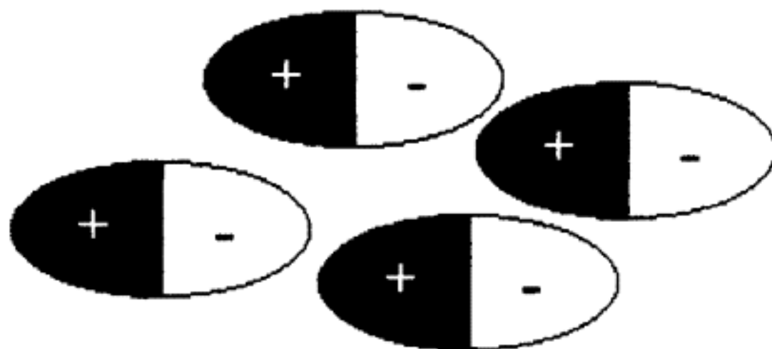
Figure 1.6. Dipole-dipole attraction
