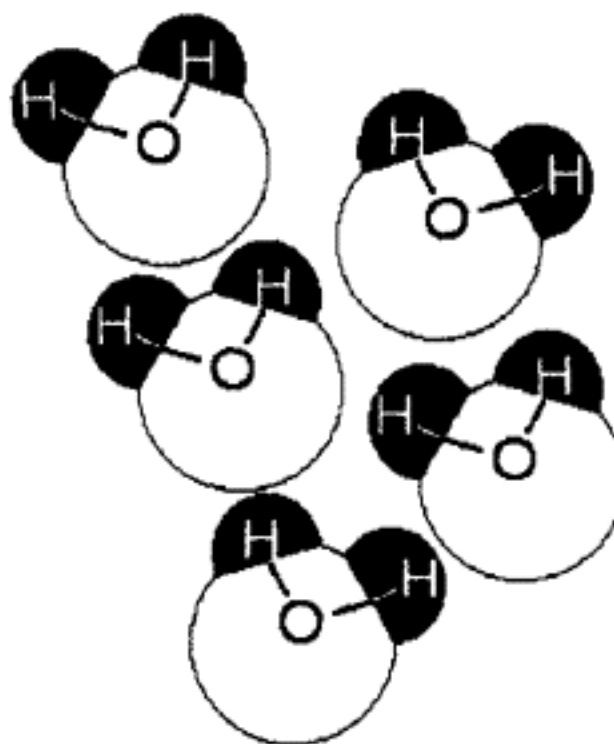
Figure 1.8. Hydrogen bonding
