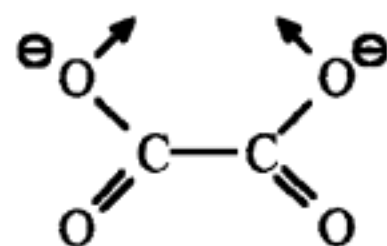
Oxalate Ion
